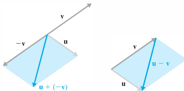
Figure 1.13 Vector subtraction
