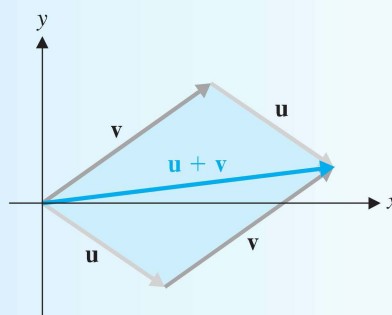
Figure 1.9 The parallelogram rule
